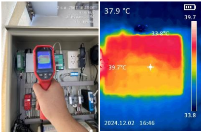
Switch Hub39.7 °C
