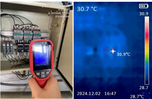
DC Panel Box No.6 30.9°C
