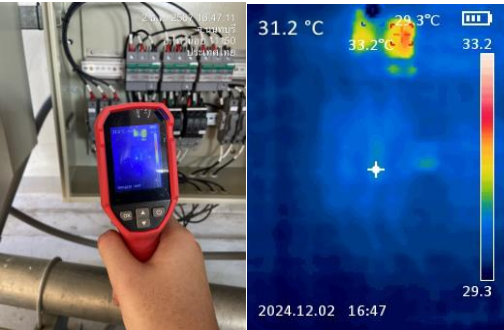
DC Panel Box No.6 33.2°C
