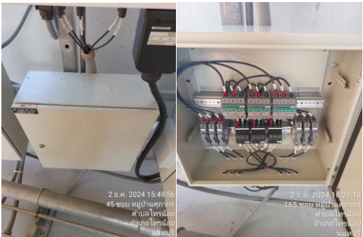
DC Panel Box No.6 20SNPB-WOC01
