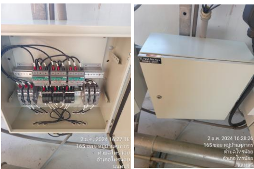
DC Panel Box No.6 20SNPB-WOC01
